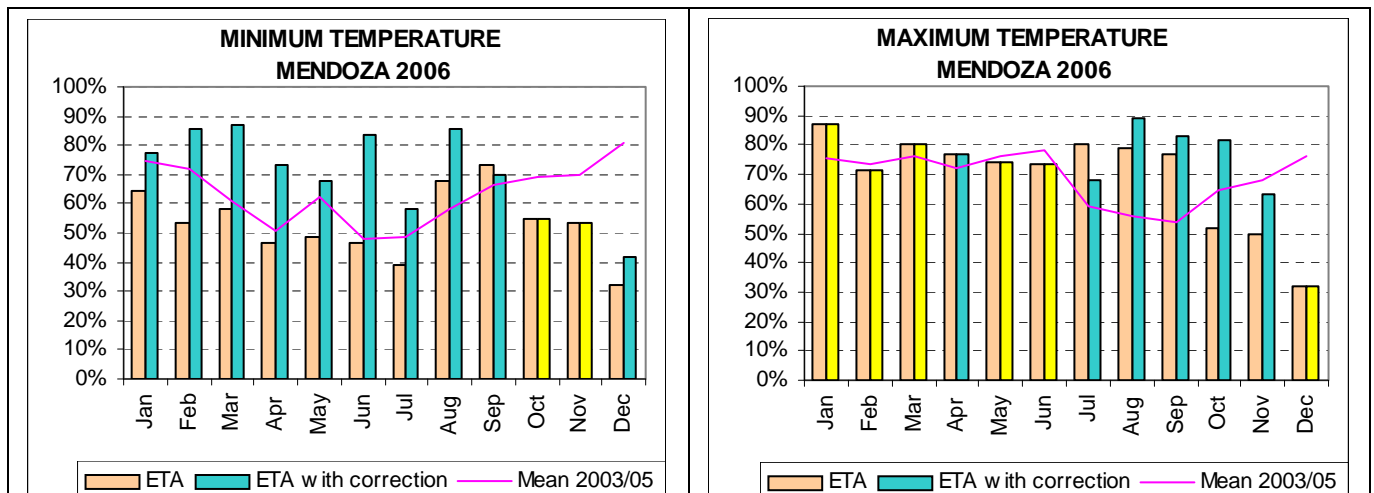
Fig. 3: Rate of hits of Maximum/Minimum Temperatures forecasts from the ETA SMN Model and the corrected forecast of the same variables. The forecasts are based on the 12 UTC cycle and are valid for the following day. Location: MENDOZA -33S -68.4W
