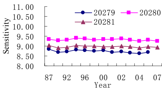
Figure 3 Stability of NIP pyrhemimeter sensitivity
