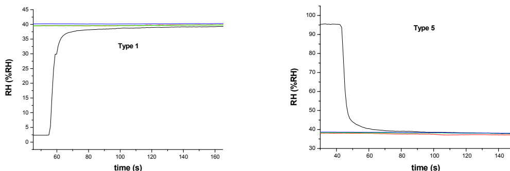
Figure 2. Time response results for a Vaisala HMT317 sensor (black line). On the y-axis the Relative Humidity in %RH derived from the measured dew point temperature and the reference temperature, on the x-axis the time in seconds. The type indication refers to the type of measurement.
