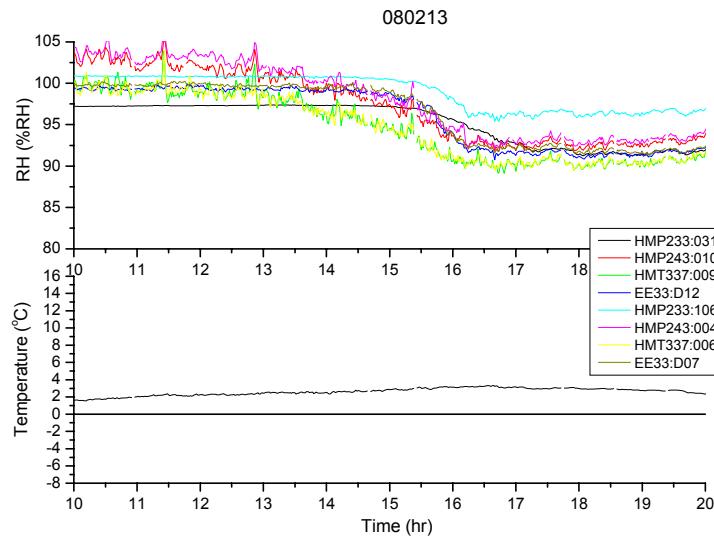
Figure 8. Results from the field test in De Bilt. Date: 13 February 2008. Upper panel: the RH from the 8 sensors (in %RH); lower panel: the average temperature of the external temperature elements (in °C). Additional measurements show that fog was present until about 13:00 when it lifted slowly. Precipitation and wind were not present.
