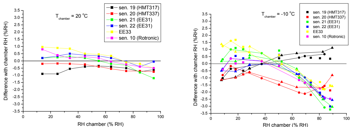
Figure 1. Example of the results from the accuracy lab tests. On the y-axis the difference in Relative Humidity between the sensor and the climate chamber, on the x-axis the humidity of the climate chamber. Left panel: climate chamber at 20 °C, right panel: climate chamber at -10 °C.
