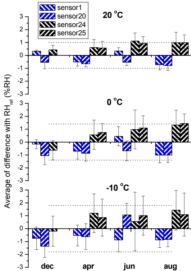
Figure 6. On the y-axes: average deviation of the difference between the sensor and the reference (in %RH) of the sensors indicated (blue: HMT 3 3 7, black: EE 3 3) for the different temperatures (20, 0 and -10 °C) and series (dec, apr, jun and aug). The standard deviation for each series is indicated by the error bar, the dashes line the uncertainty of the measurement for the temperature in question.
