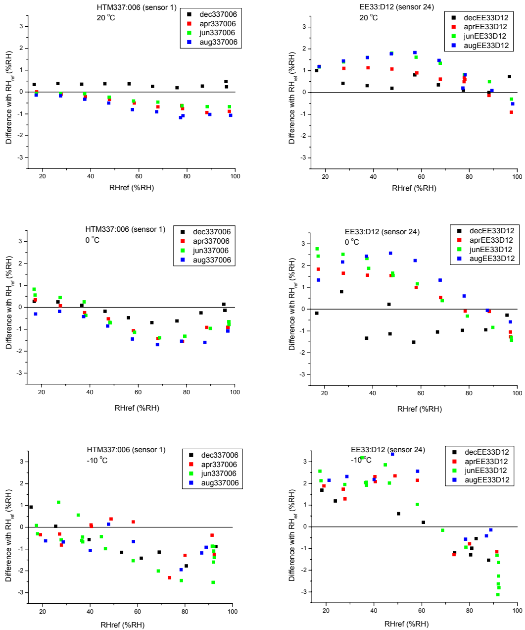
Figure 5. Example of the results of the lab checks during the field test for one HMT337 sensor (left figures) and one EE33 sensor (right figures), including the earlier calibrations (“dec”, black symbols). “apr” is after 2 months of field test (red), “jun” after 4 months (green) and “aug” after 6 months (blue). For each measurement, the temperature is indicated. On the y-axis the difference in Relative Humidity between the sensor and the climate chamber is indicated (in %RH), on the x-axis the humidity of the climate chamber (in %RH).
