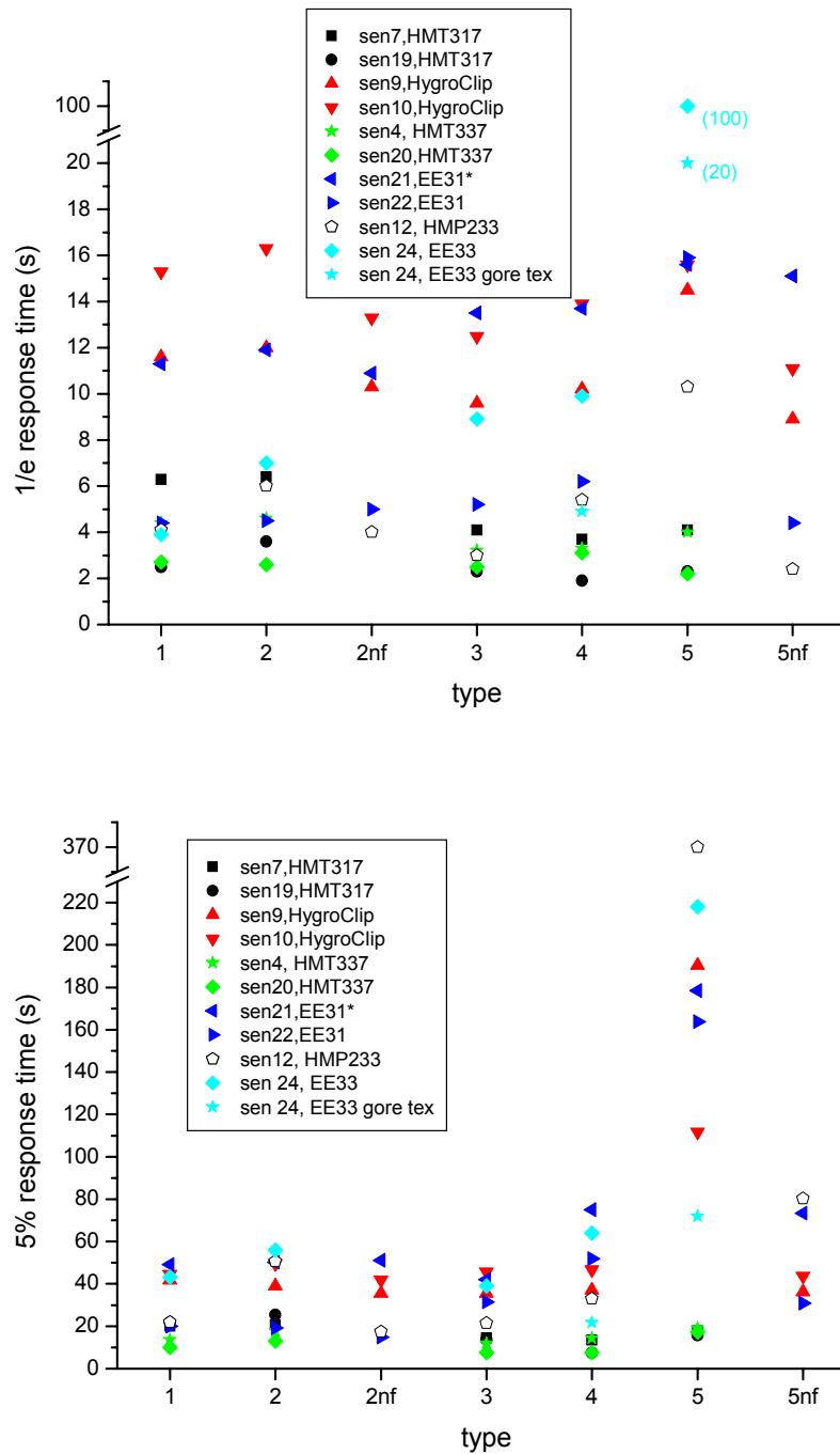
Figure 3. 1/e response times (upper plot) and 5 % response times (lower plot) as a function of measurement type for the sensors indicated. “nf” means no protective filter present (only for the non-heated sensors). Same colour means same sensor type. The EE31* has a special coating.
