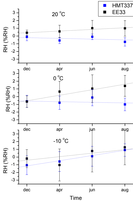
Figure 7. Fits based on the data of Figure 6, where the data for the two sensors of each type are combined. On the y-axes: average deviation of the difference between the sensor and the reference (in %RH) of the sensors indicated (blue: HMT337, black: EE33) for the different temperatures (20, 0 and -10 °C) and series (dec, apr, jun and aug). The standard deviation for each series is indicated by the error bar.
