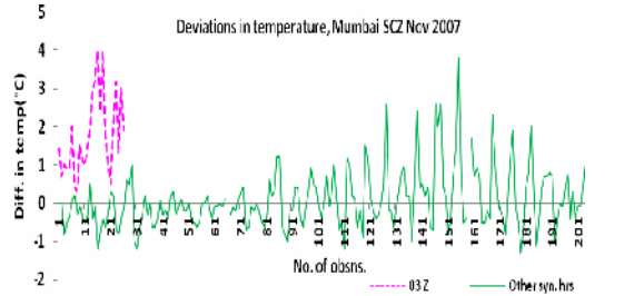
Fig.11 Variation in meteorological parameters for Mumbai SCZ Nov 2007
