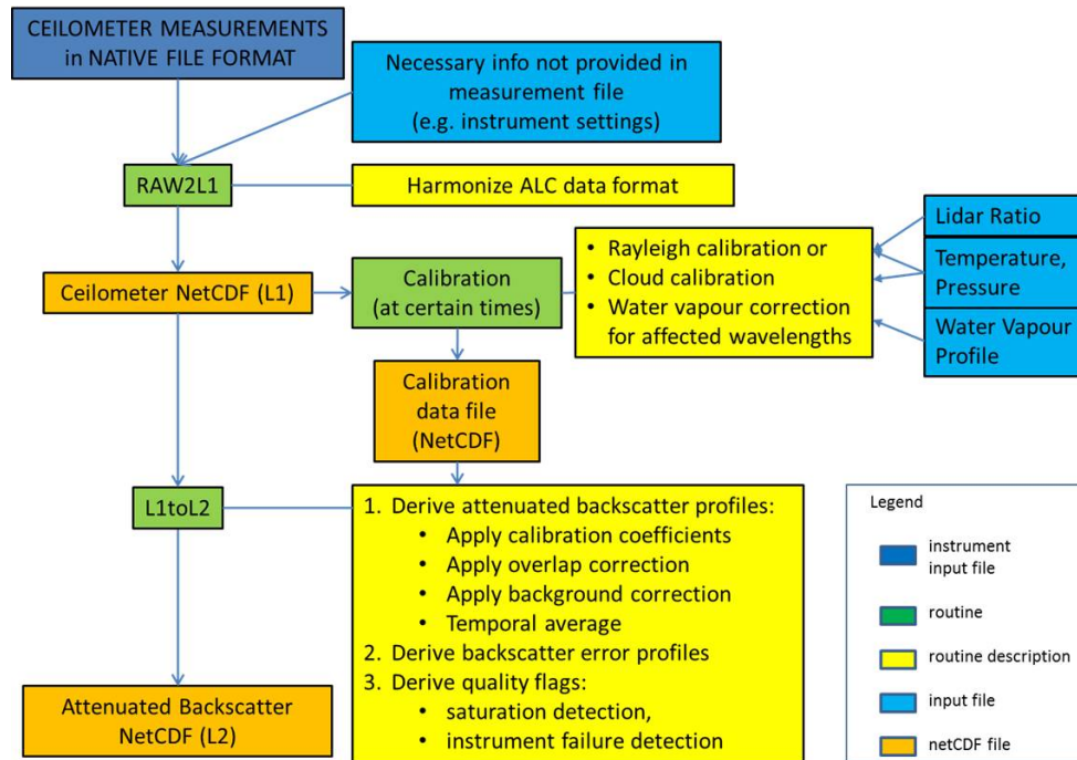
Figure 4: Schematic of the production chain of attenuated backscatter coefficient from raw data.
