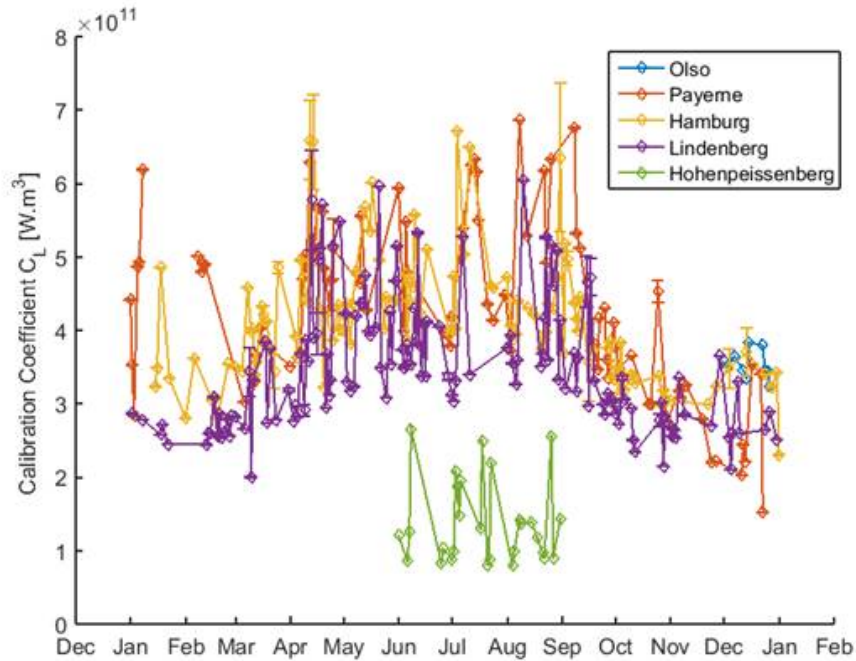
Figure 1: Time series of the calibration factor of 5 ceilometers of type CHM15k derived with the Rayleigh method (see text).
