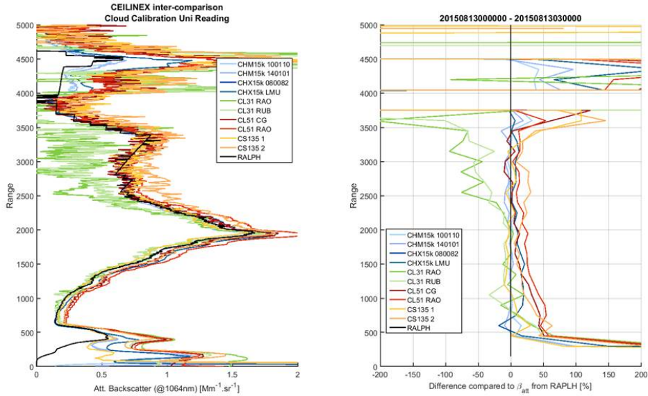
Figure 3: Left panel: profiles of attenuated backscatter coefficient at 1064 nm as measured with different ceilometers. Right panel: difference in attenuated backscatter coefficient at 1064 nm between the ceilometers and the research lidar Ralph.
