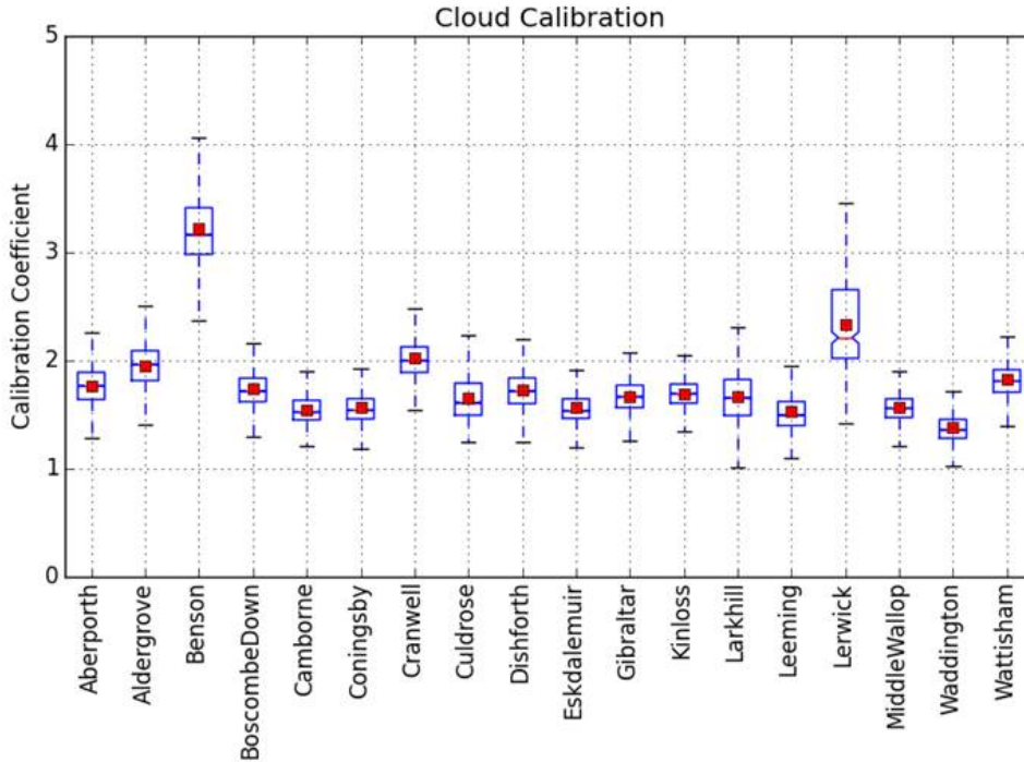
Figure 2: Average and spread of the calibration coefficient of the Vaisala/CL31 network of the Met Office derived with the cloud method calculated over 1 year (see text).
