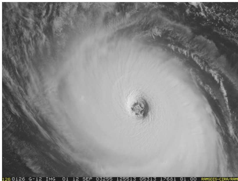
Figure 2.6 Mesovortices within the eye of Hurricane Isabel (2003).
